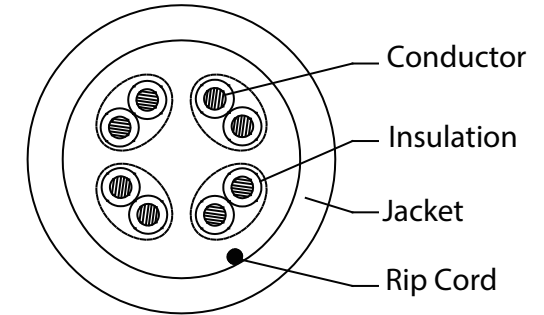
Cross Section
