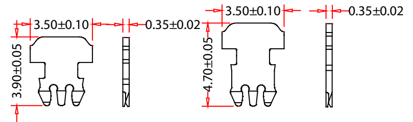
3 Prongs for Stranded Wire
