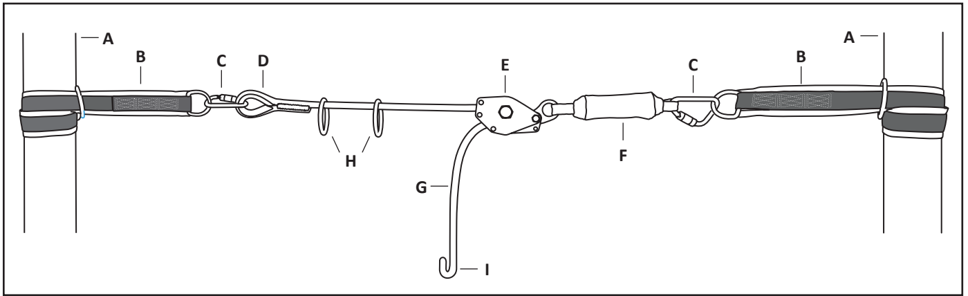
Figure 1: About FallTech Kernmantle Horizontal Lifeline
