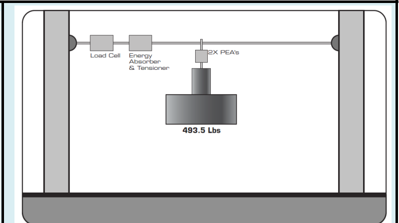
Figure 2: 2-Person Drop Test Configuration
