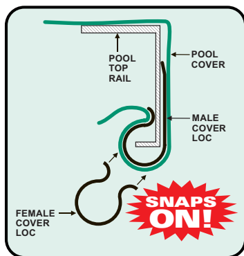
Installation Diagram
