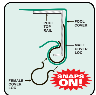
Installation Diagram
