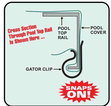
Installation Diagram
