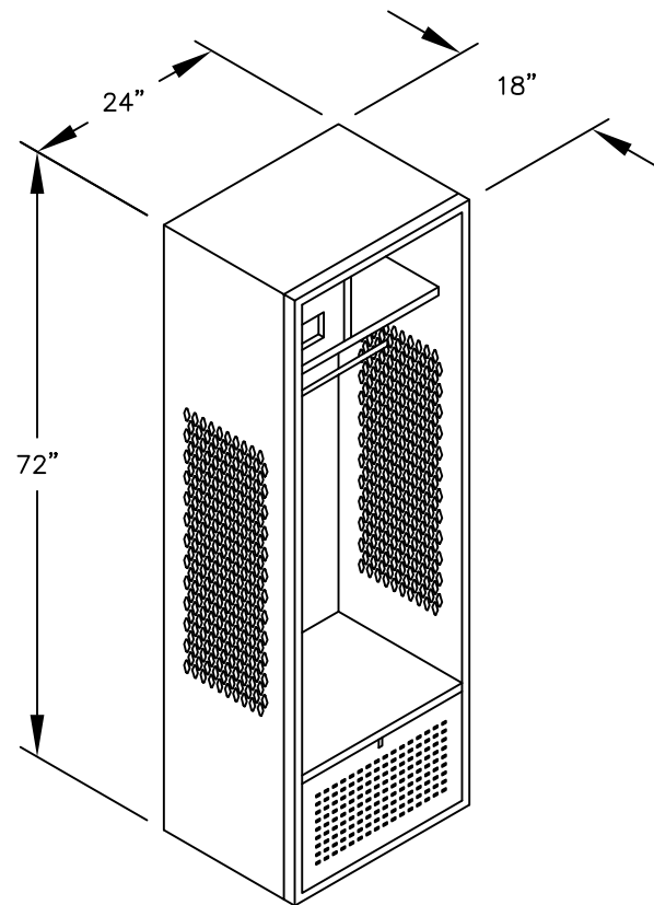
MODEL #70018 24" WIDE OPEN ACCESS STANDARD LOCKER
