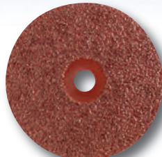
Zone Coated: Grain is placed, leaving a clear Zone around the arbor. Easier to lock on a grinder and provides a tighter fit. Excellent on coarse grits, where grain can be a hindrance.
