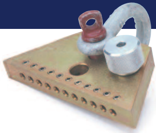
UNI-1080 Uni-Clamp multiple stud puller Parts: 1081 - screws only, pkg of 8 1082 - screw wrench only
