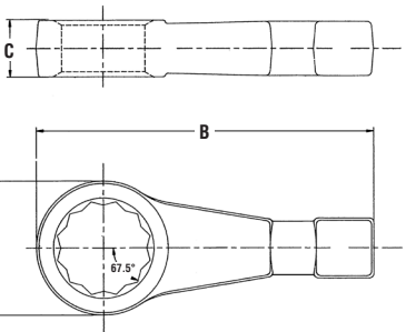
Roughneck "Hammer Wrench" Straight Pattern — 12 Point Alloy Steel — Drop Forged SAE and Metric
