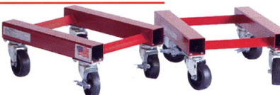
77788 Wheel Dollies: 4" heavy duty swivel wheels (two locking) / Fully welded all-steel frame / 2 piece set / Each holds 1500 lbs.
