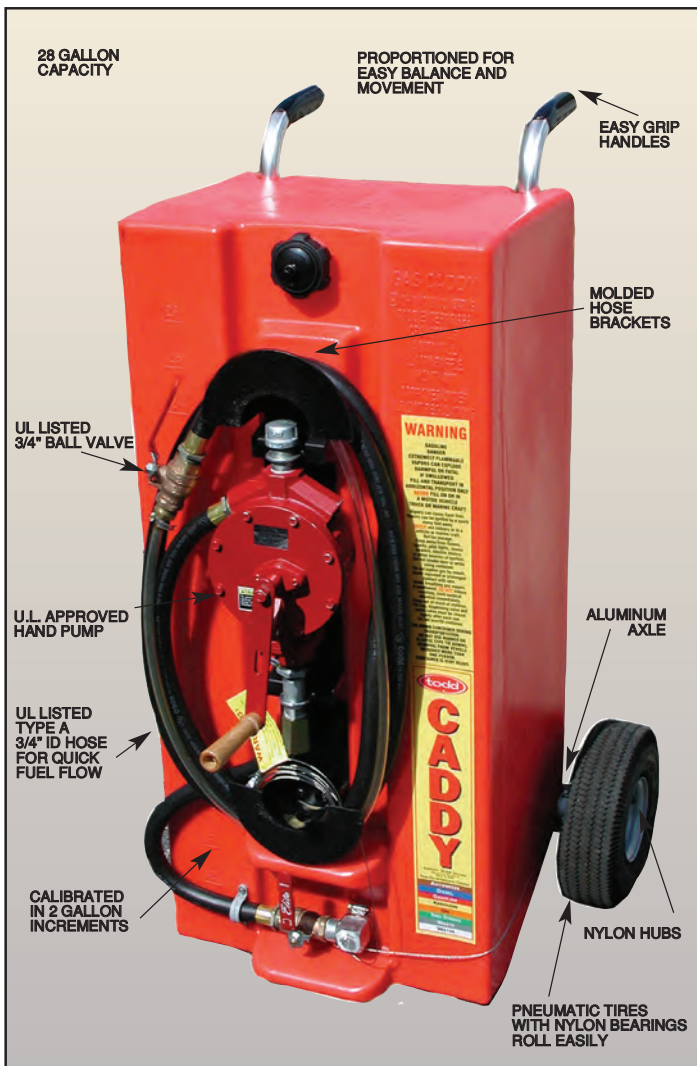
Shown with Industrial Pump and Evacuation Kit P/N 2403IPQD
