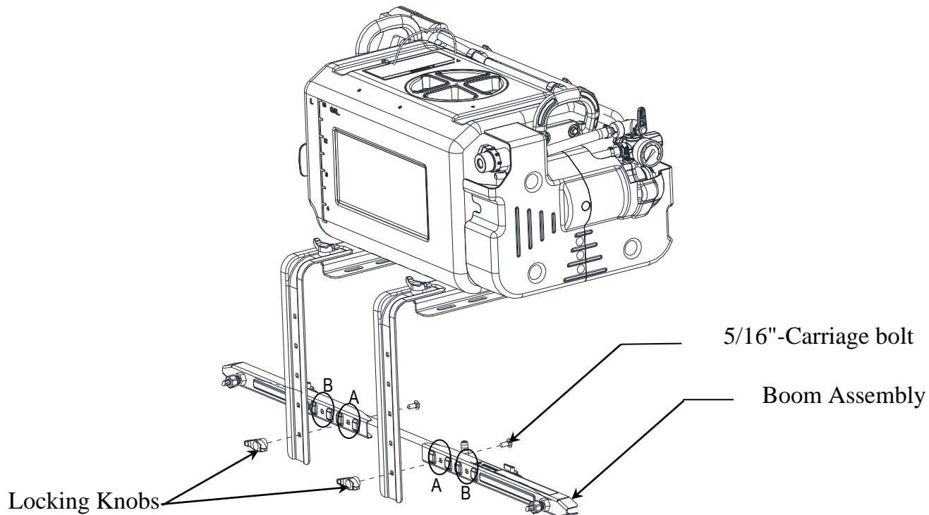
5/16"-Carriage bolt 82088 (Qty 2)
