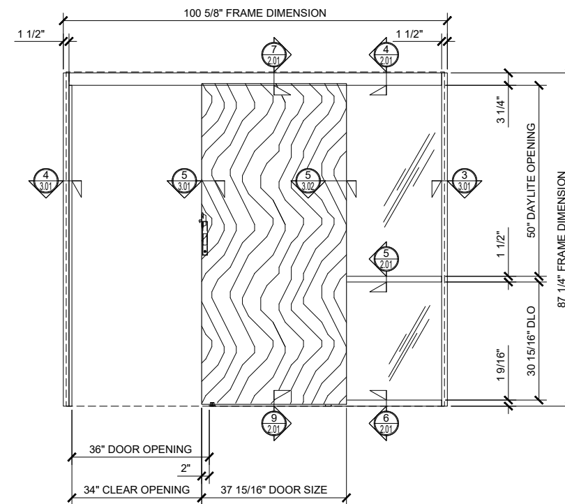
② SINGLE SLIDER WITH DOUBLE SIDELITE (OPEN)
