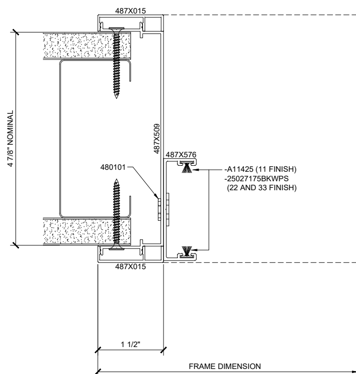
④ SERIES 487 OPS INTEGRATED SLIDER STRIKE JAMB DETAIL (OPEN)
