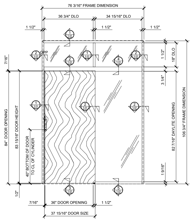
③ SINGLE SLIDER WITH TRANSOM AND SINGLE SIDELITE (CLOSED) ARCH REF: NONE 3/4"=1'-0"
