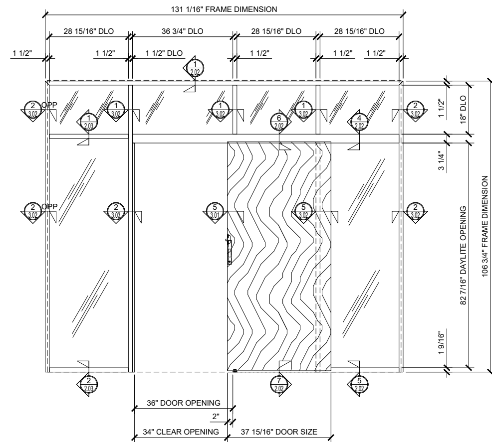
4 SINGLE SLIDER WITH TRANSOM AND DOUBLE SIDELITE (OPEN)
