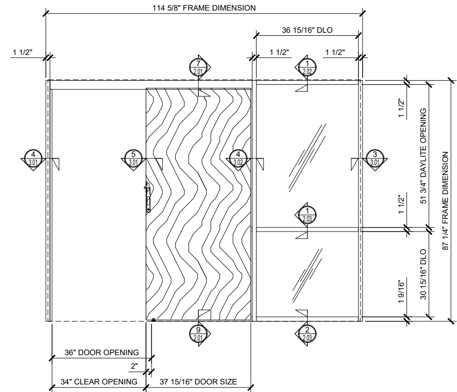
② SINGLE SLIDER WITH DOUBLE SIDELITE (OPEN)
