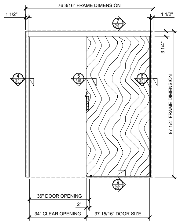
② SINGLE SLIDER WITH SINGLE SIDELITE (OPEN) ARCH REF: NONE 3/4"=1'-0"
