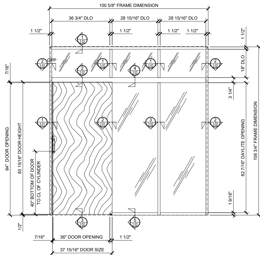
③ SINGLE SLIDER WITH TRANSOM AND DOUBLE SIDELITE (CLOSED)
