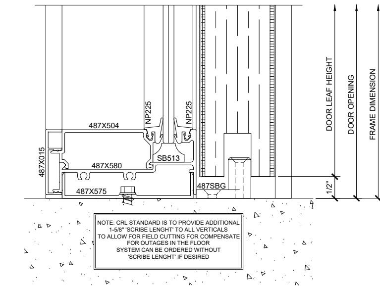
9 SILL AT SLIDER SIDELITE (DOOR OPEN) ARCH REF: 1'-0"=1'-0"
