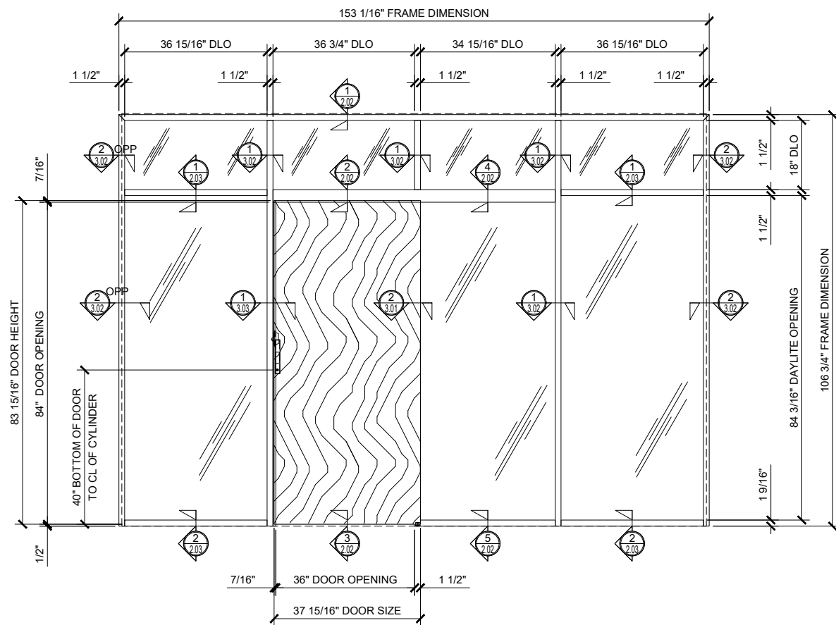
③ SINGLE SLIDER WITH TRANSOM AND DOUBLE SIDELITE (CLOSED)
