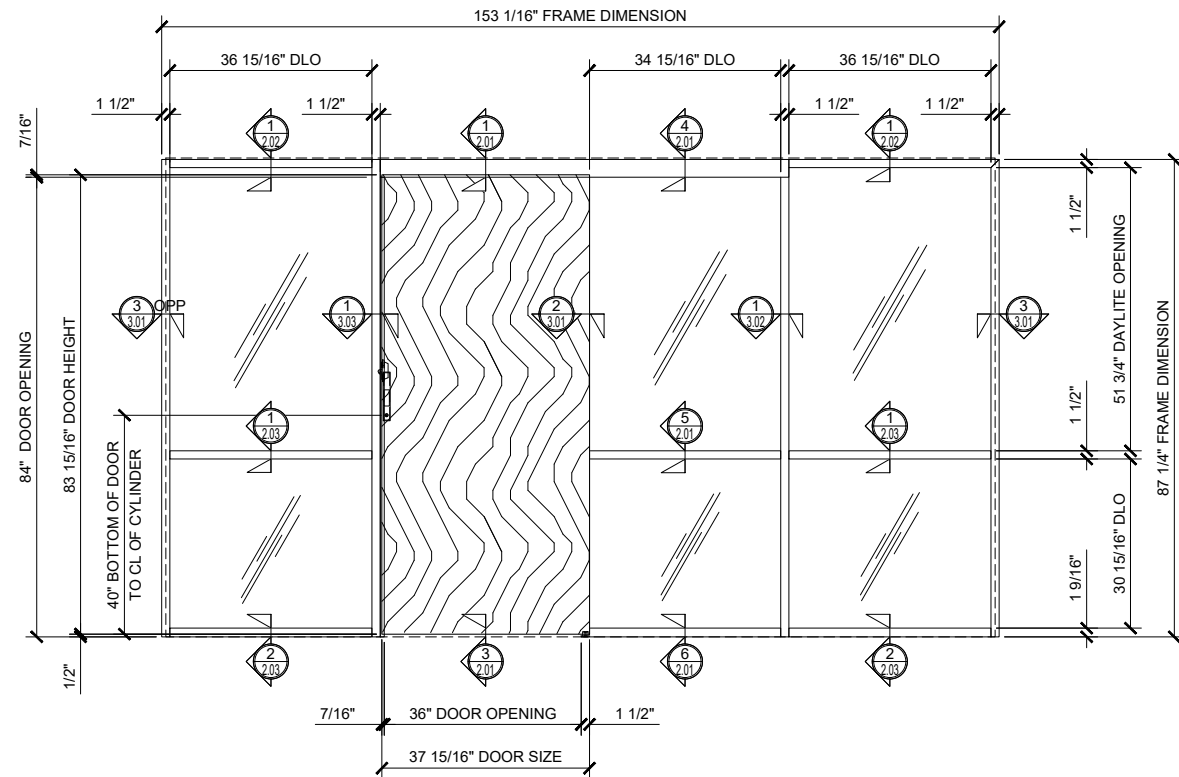
① SINGLE SLIDER WITH DOUBLE SIDELITE (CLOSED)
