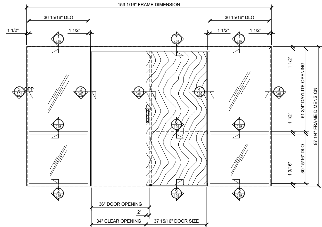
② SINGLE SLIDER WITH DOUBLE SIDELITE (OPEN)
