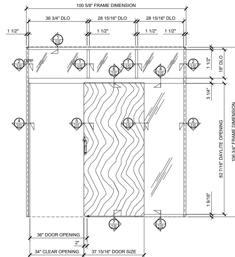
④ SINGLE SLIDER WITH TRANSOM AND DOUBLE SIDELITE (OPEN)
