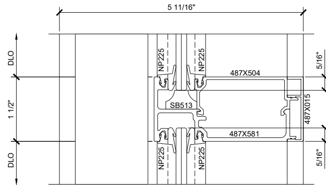
5 MUNTIN AT SLIDER SIDELITE (DOOR CLOSED) ARCH REF: 1'-0"=1'-0"
