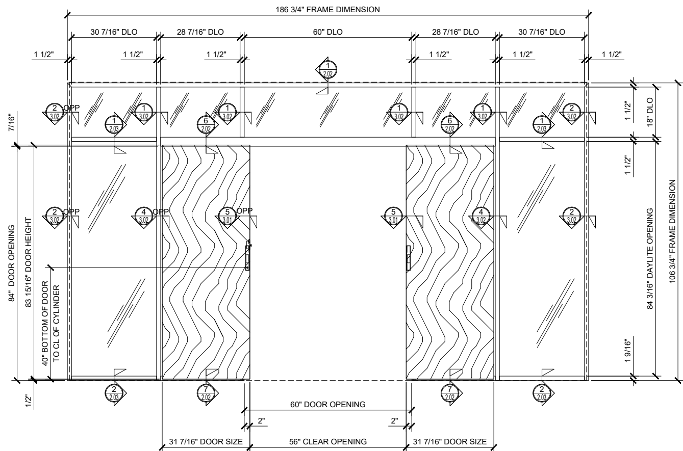
4 BI-PART SLIDER WITH TRANSOM AND SINGLE SIDELITES (OPEN)
