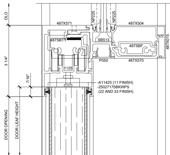
② TRANSOM DETAIL AT SLIDER DOOR OPENING
