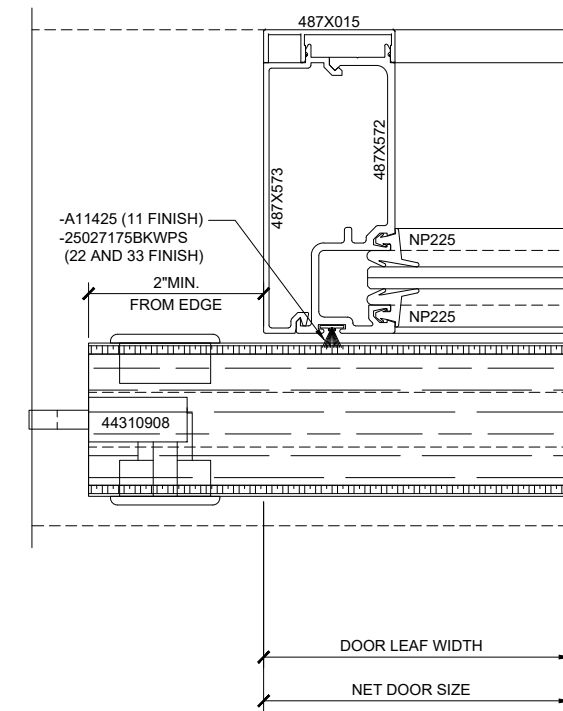
⑤ SERIES 487 OPS INTEGRATED SLIDER INTERMEDIATE JAMB DETAIL (OPEN)
