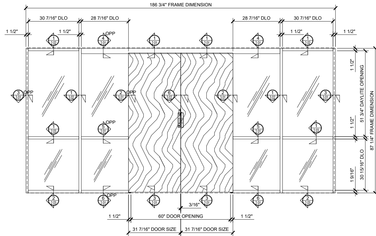
1 BI-PART SLIDER WITH SINGLE SIDELITES (CLOSED)
