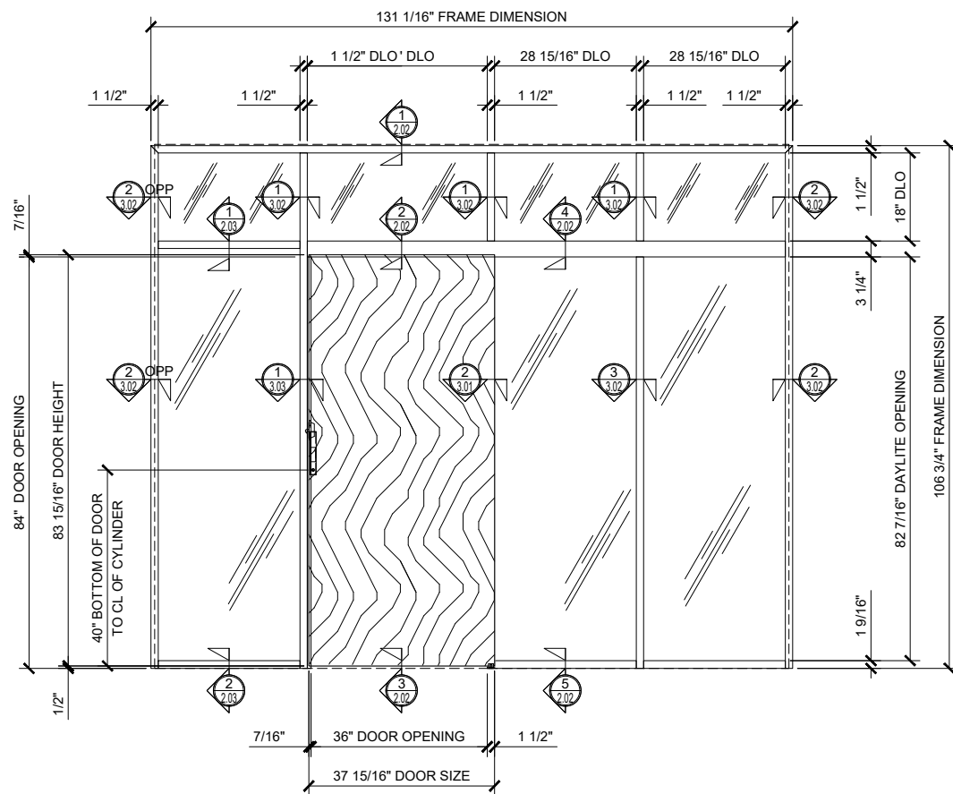
3 SINGLE SLIDER WITH TRANSOM AND DOUBLE SIDELITE (CLOSED)
