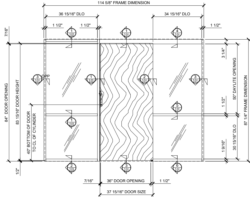
① SINGLE SLIDER WITH SINGLE SIDELITE (CLOSED)
