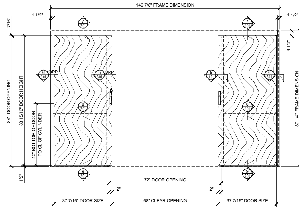
② BI-PART SLIDER WITH SINGLE SIDELITES (OPEN) ARCH REF: NONE 3/4"=1'-0"
