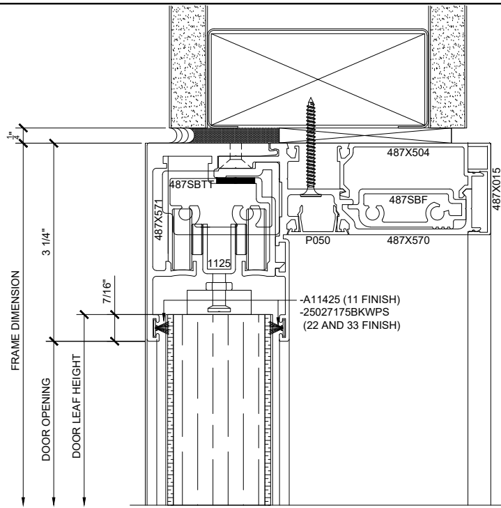
1 HEAD DETAIL AT SLIDER DOOR OPENING ARCH REF: 1'-0"=1'-0"
