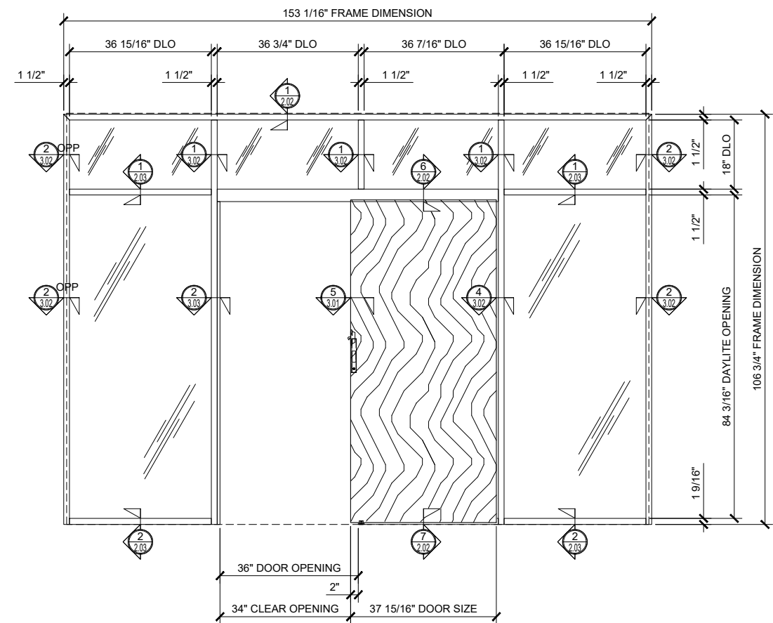
④ SINGLE SLIDER WITH TRANSOM AND DOUBLE SIDELITE (OPEN)
