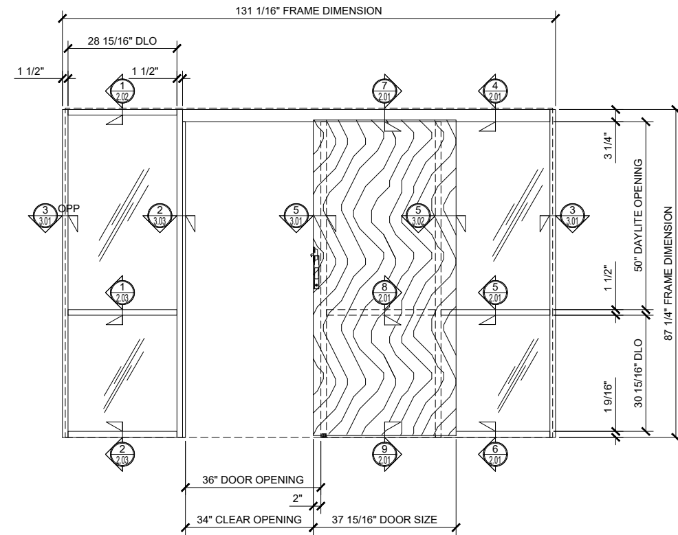
2 SINGLE SLIDER WITH DOUBLE SIDELITE (OPEN)
