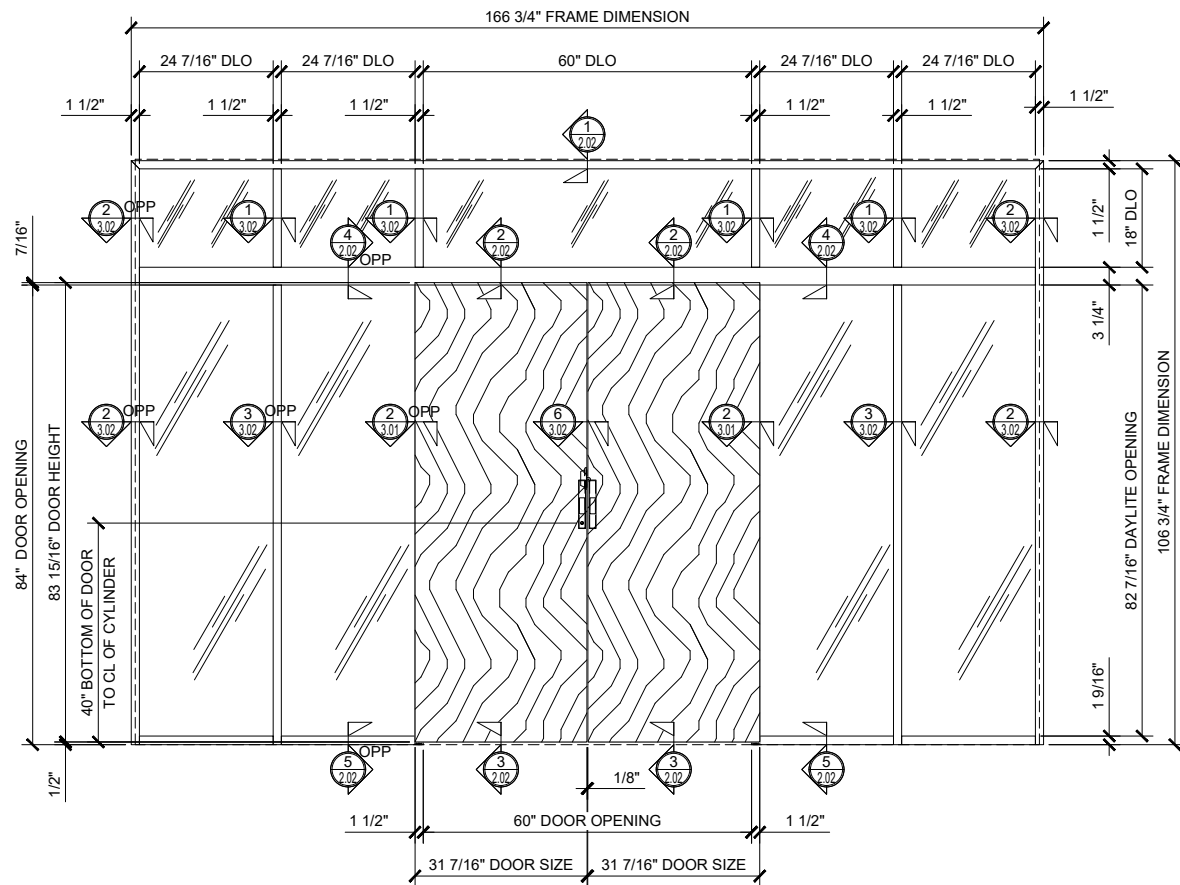
③ BI-PART SLIDER WITH TRANSOM AND SINGLE SIDELITES (CLOSED)
