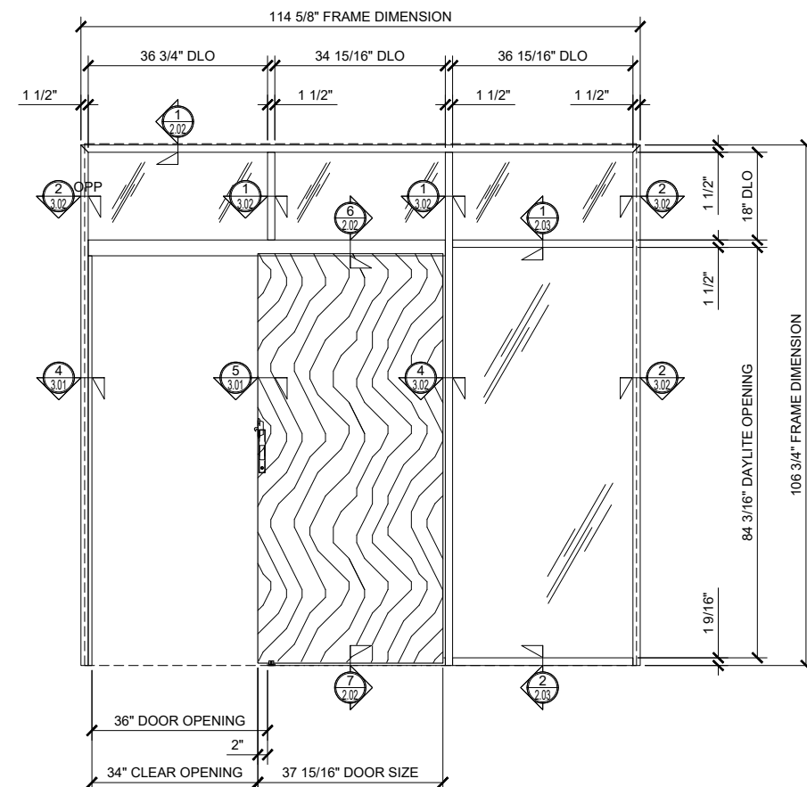
④ SINGLE SLIDER WITH TRANSOM AND DOUBLE SIDELITE (OPEN)
