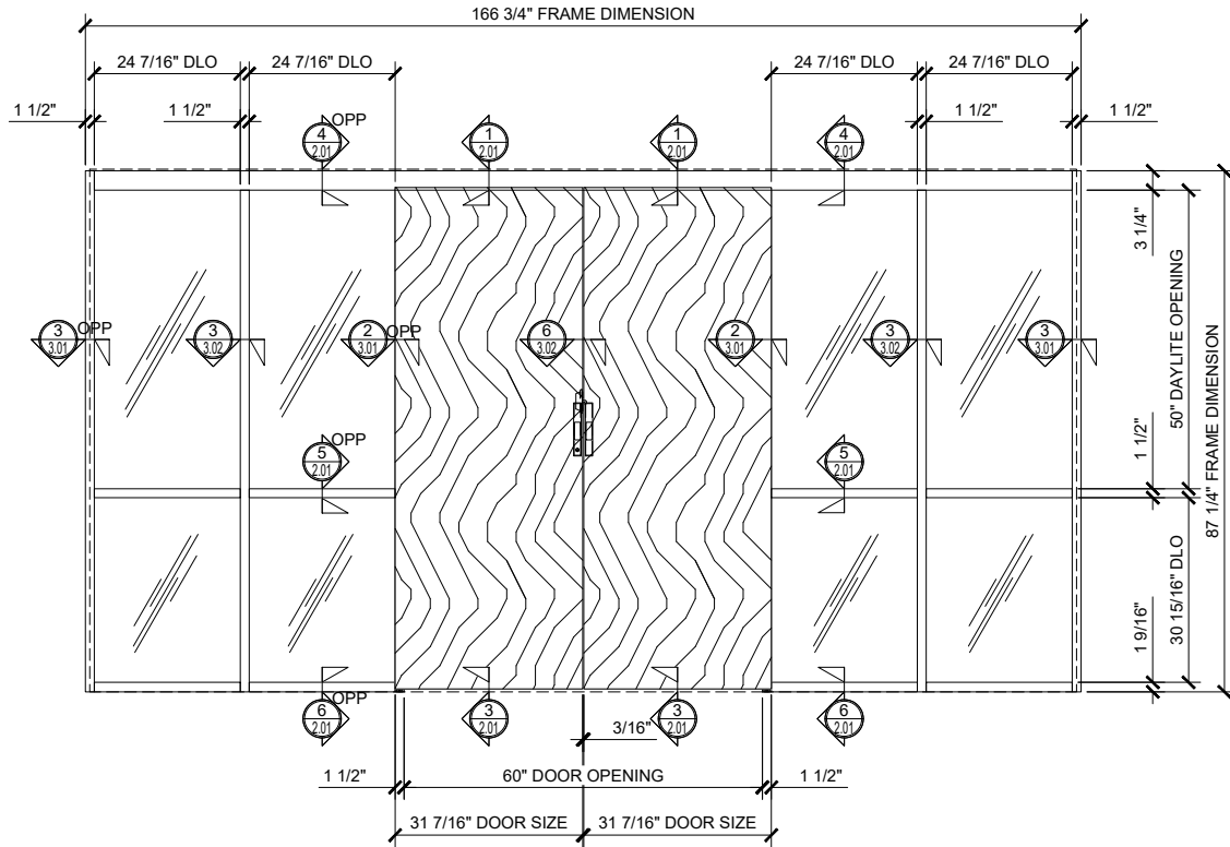
① BI-PART SLIDER WITH SINGLE SIDELITES (CLOSED)
