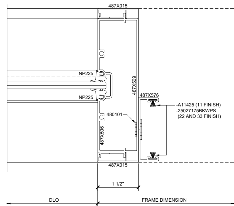
② SERIES 487 OPS INTEGRATED SLIDER TRANSITION VERTICAL-STANDARD TO STRIKE JAMB (OPEN)
