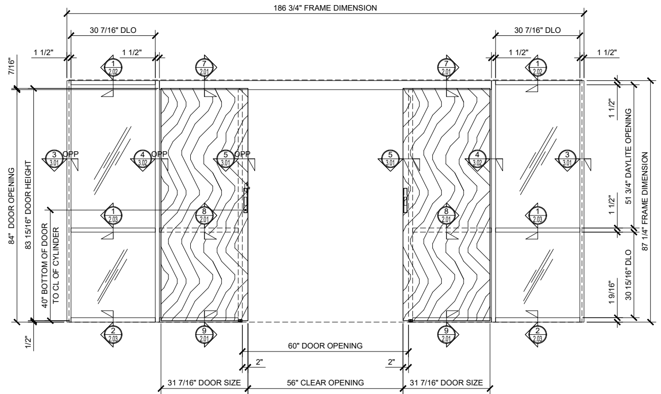
2 BI-PART SLIDER WITH SINGLE SIDELITES (OPEN)
