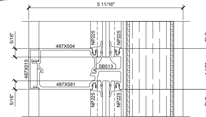
8 MUNTIN AT SLIDER SIDELITE (DOOR OPEN) ARCH REF: 1'-0"=1'-0"
