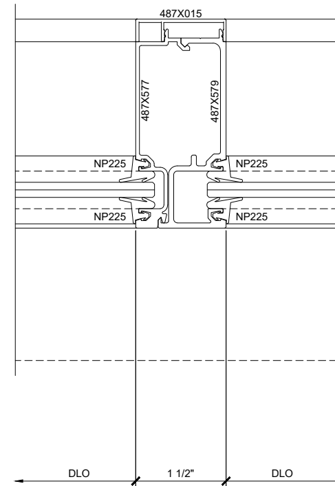
③ SERIES 487 OPS INTEGRATED SLIDER BY-PASS INTERMEDIATE VERTICAL DETAIL (CLOSED) ARCH REF: 1'-0"=1'-0"
