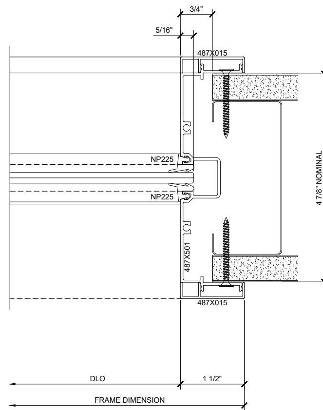
③ SERIES 487 OPS INTEGRATED SLIDER WALL JAMB DETAIL (CLOSED)
