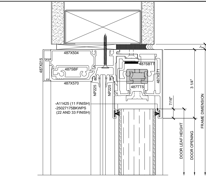
7 HEAD DETAIL AT SLIDER SIDELITE (DOOR OPEN) ARCH REF: 1'-0"=1'-0"
