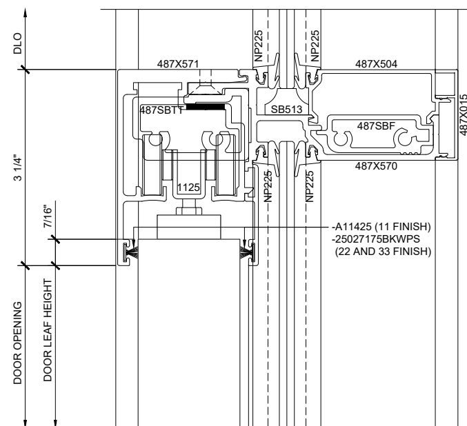
④ TRANSOM DETAIL AT SLIDER SIDELITE (DOOR CLOSED)
