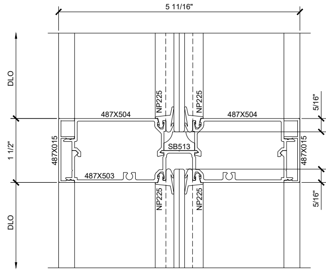
① SERIES 487 OPS TYP HORIZONTAL DETAIL ARCH REF: 1'-0"=1'-0"
