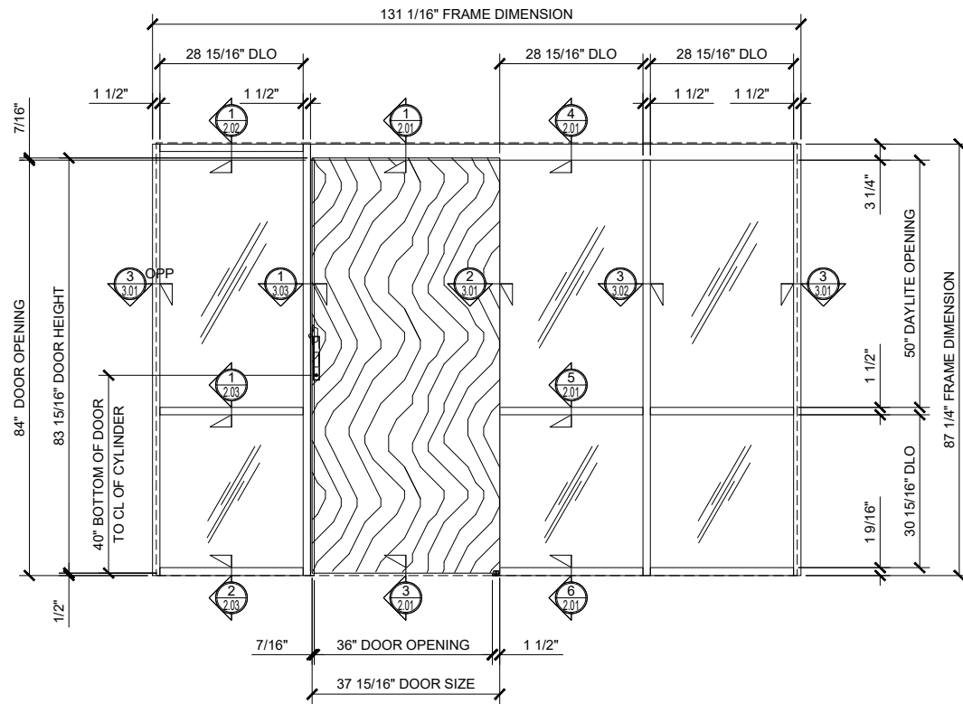
1 SINGLE SLIDER WITH DOUBLE SIDELITE (CLOSED)
