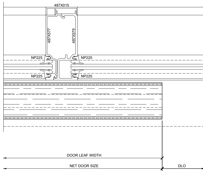
⑤ SERIES 487 OPS INTEGRATED SLIDER SHALLOW VERTICAL DETAIL (OPEN) ARCH REF: 1'-0"=1'-0"
