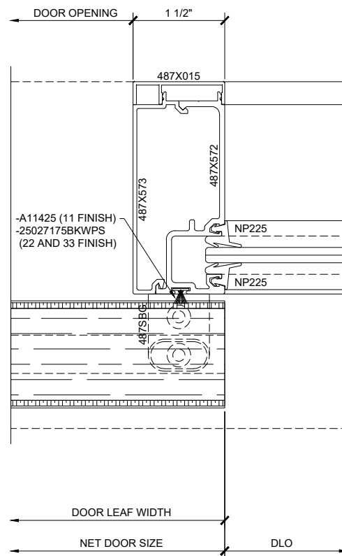
② SERIES 487 OPS INTEGRATED SLIDER INTERMEDIATE JAMB DETAIL (CLOSED)
