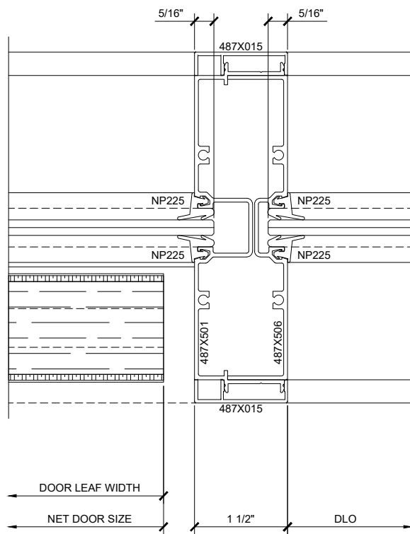
④ SERIES 487 OPS INTEGRATED SLIDER TRANSITION VERTICAL-SLIDER TO STANDARD (OPEN) ARCH REF: 1'-0"=1'-0"
