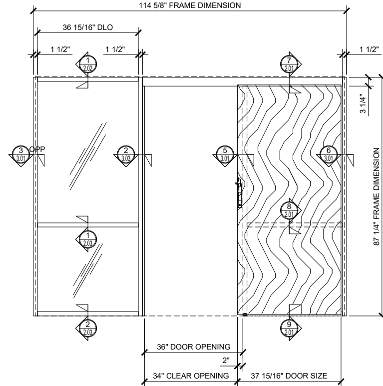
② SINGLE SLIDER WITH SINGLE SIDELITE (OPEN)
