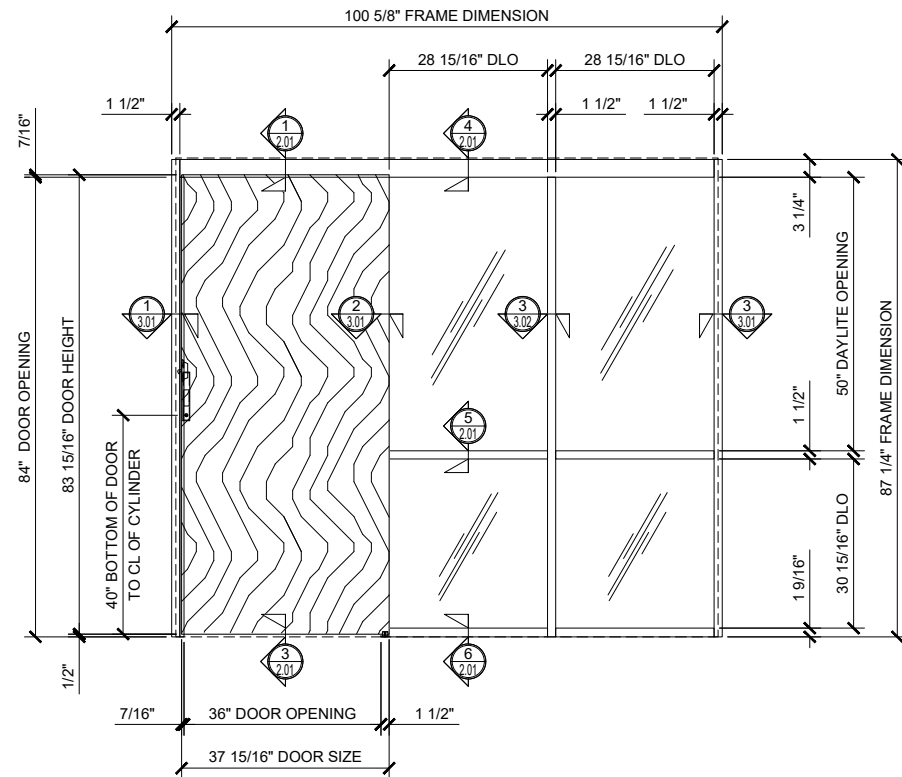
① SINGLE SLIDER WITH DOUBLE SIDELITE (CLOSED)
