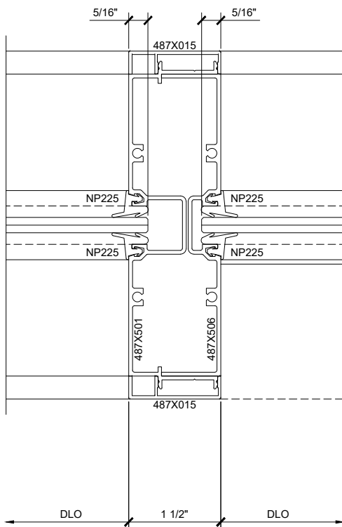
① SERIES 487 OPS INTEGRATED SLIDER TRANSITION VERTICAL-SLIDER TO STANDARD (CLOSED) ARCH REF: 1'-0"=1'-0"
