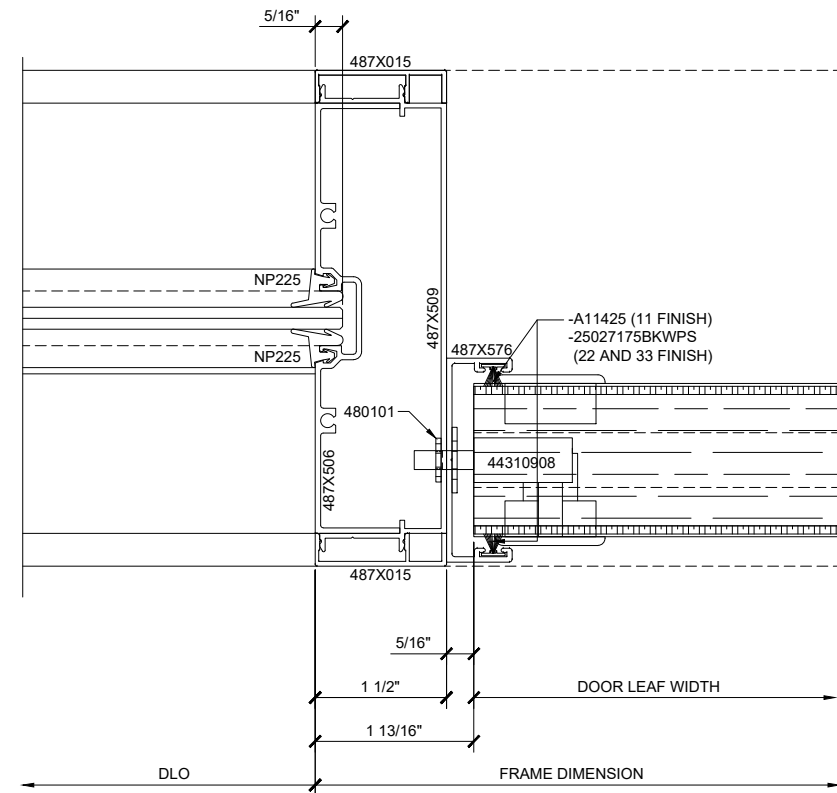
① SERIES 487 OPS INTEGRATED SLIDER TRANSITION VERTICAL-STANDARD TO STRIKE JAMB (CLOSED)
