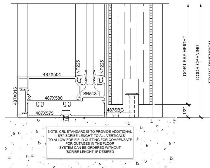
⑦ SILL AT SLIDER DOOR SIDELITE (DOOR OPEN)
