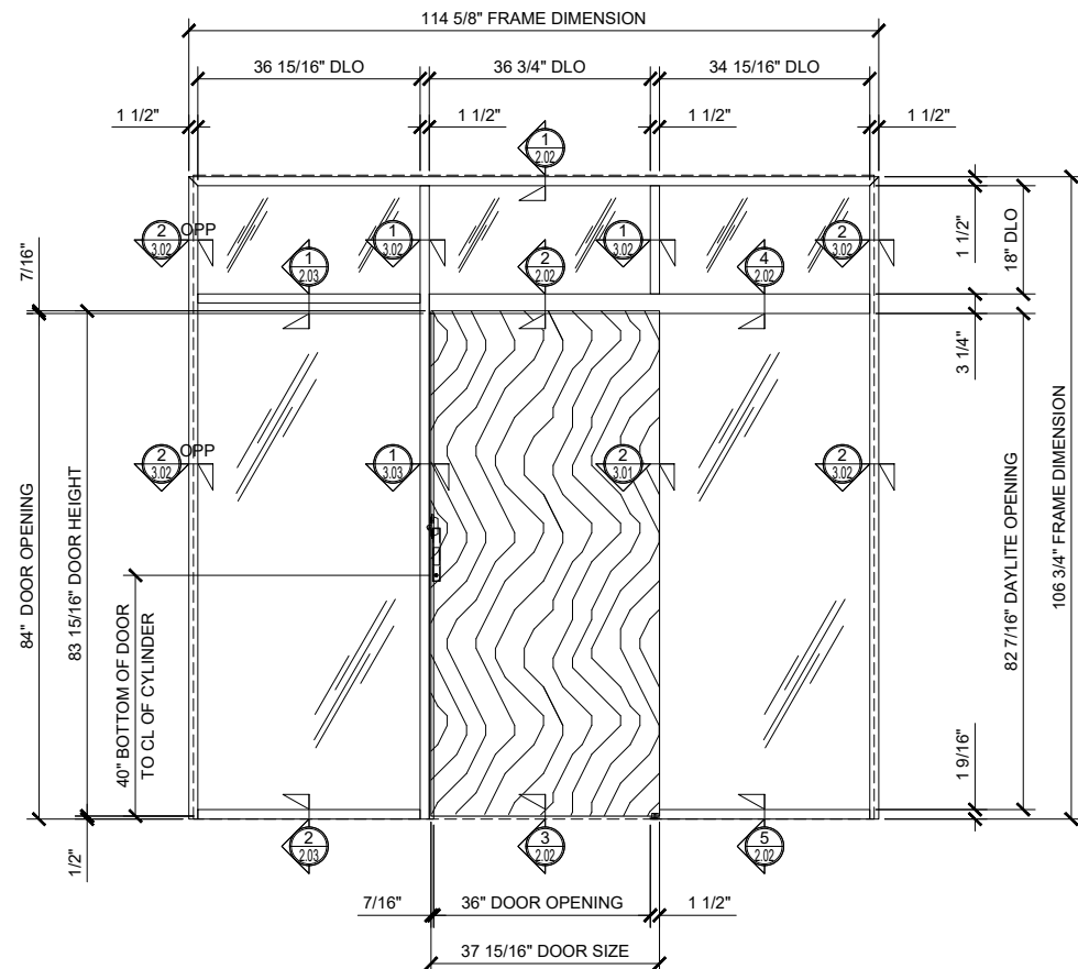
③ SINGLE SLIDER WITH TRANSOM AND SINGLE SIDELITE (CLOSED)
