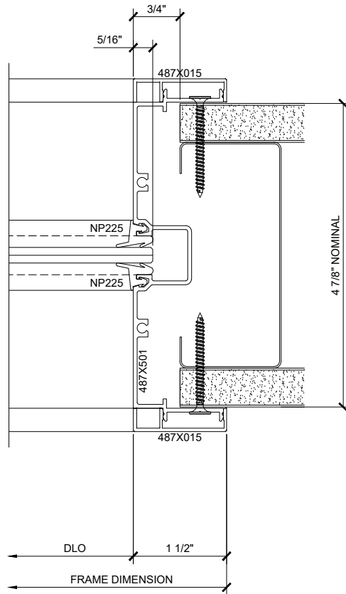
② SERIES 487 OPS STANDARD JAMB DETAIL ARCH REF: 1'-0"=1'-0"
