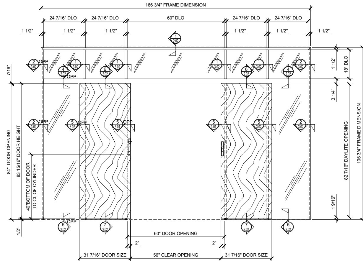
④ BI-PART SLIDER WITH TRANSOM AND SINGLE SIDELITES (OPEN)
