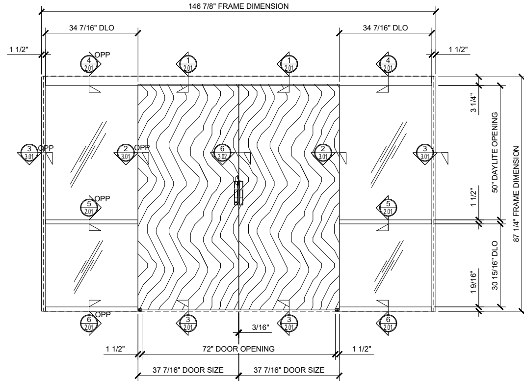
① BI-PART SLIDER WITH SINGLE SIDELITES (CLOSED) ARCH REF: NONE 3/4"=1'-0"
