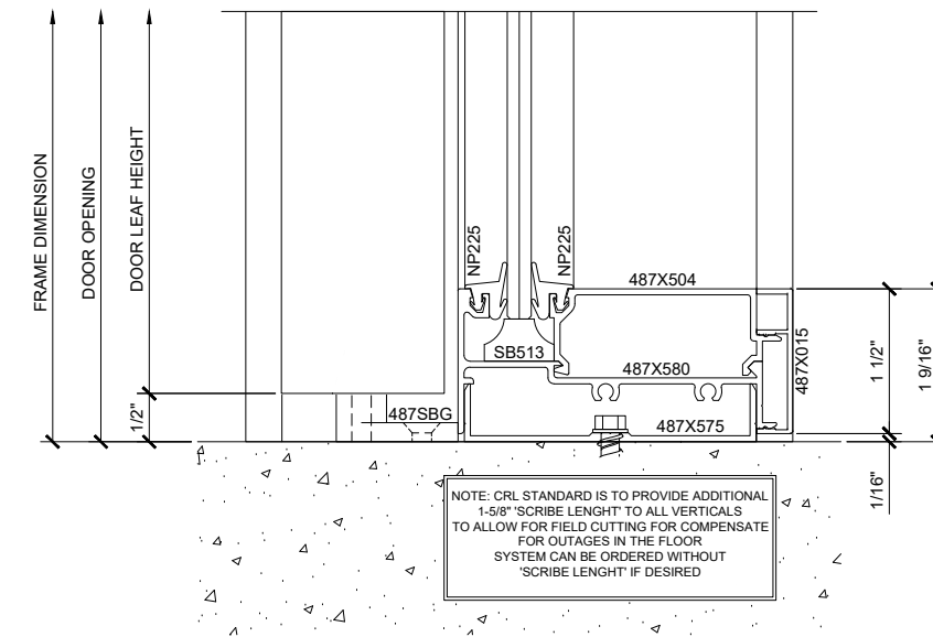
6 SILL AT SLIDER SIDELITE (DOOR CLOSED) ARCH REF: 1'-0"=1'-0"
