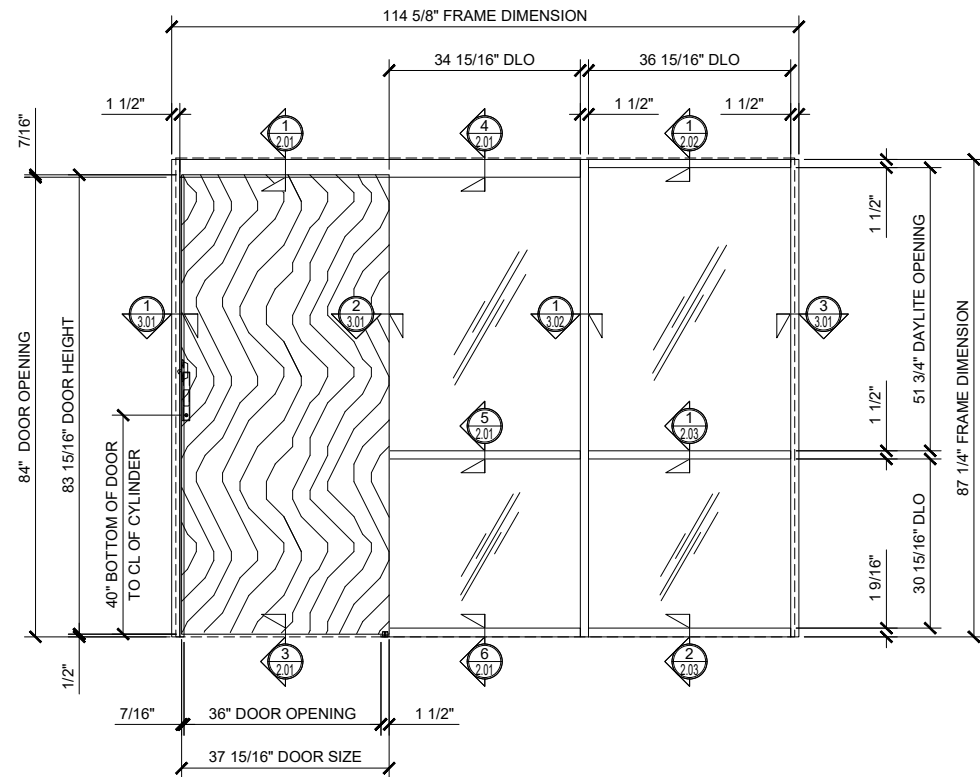
① SINGLE SLIDER WITH DOUBLE SIDELITE (CLOSED)
