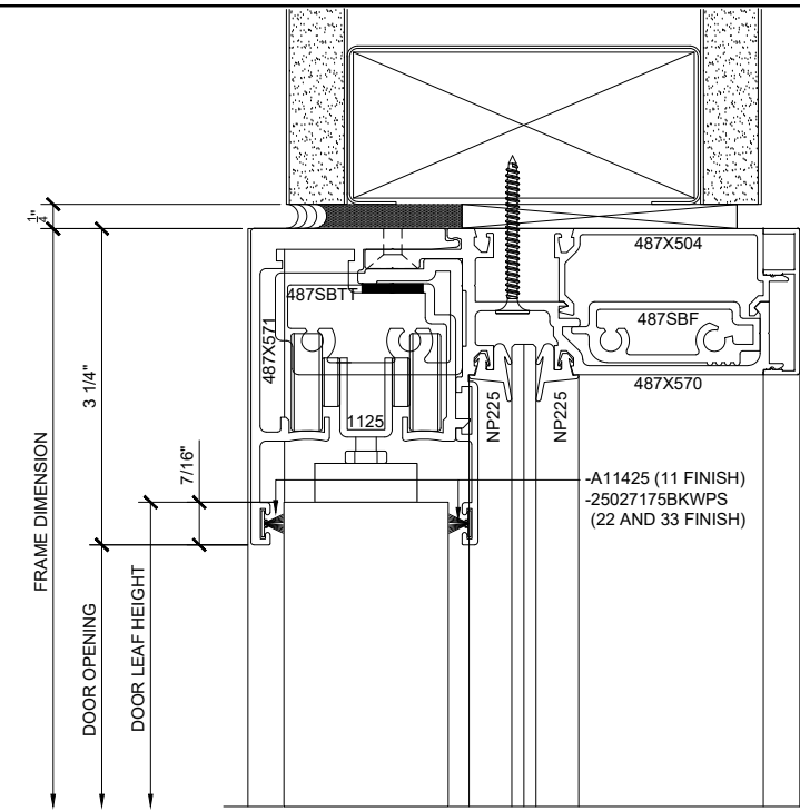
4 HEAD DETAIL AT SLIDER SIDELITE (DOOR CLOSED) ARCH REF: 1'-0"=1'-0"
