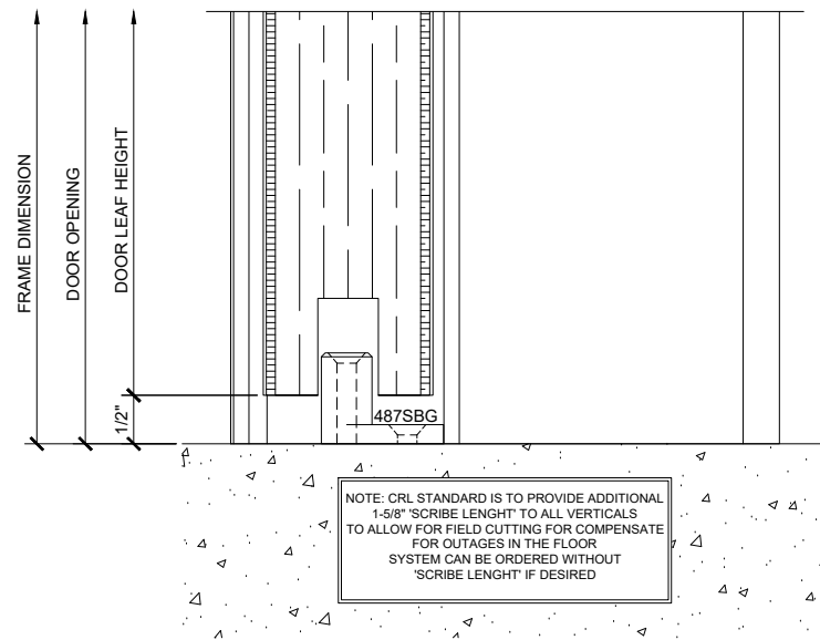
3 SILL AT SLIDER DOOR OPENING ARCH REF: 1'-0"=1'-0"
