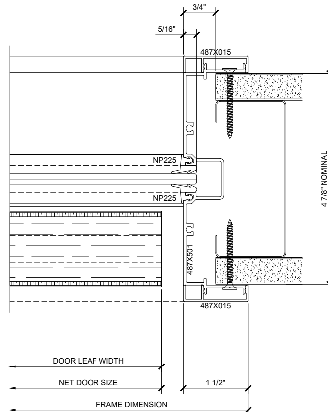
⑥ SERIES 487 OPS INTEGRATED SLIDER WALL JAMB DETAIL (OPEN)
