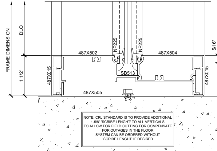
② SERIES 487 OPS TYP SILL AT FLOOR DETAIL ARCH REF: 1'-0"=1'-0"
