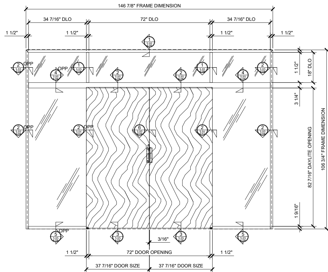
③ BI-PART SLIDER WITH TRANSOM AND SINGLE SIDELITES (CLOSED) ARCH REF: NONE 3/4"=1'-0"
