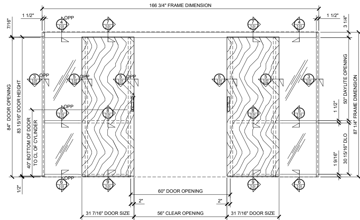
② BI-PART SLIDER WITH SINGLE SIDELITES (OPEN)
