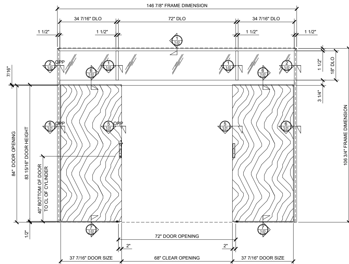
④ BI-PART SLIDER WITH TRANSOM AND SINGLE SIDELITES (OPEN) ARCH REF: NONE 3/4"=1'-0"
