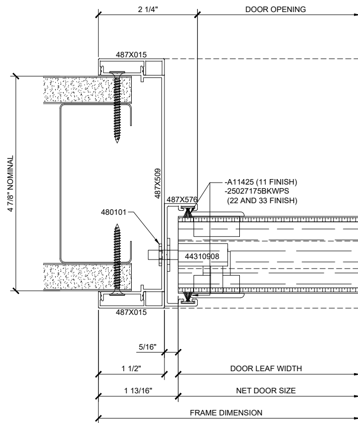
① SERIES 487 OPS INTEGRATED SLIDER STRIKE JAMB DETAIL (CLOSED)
