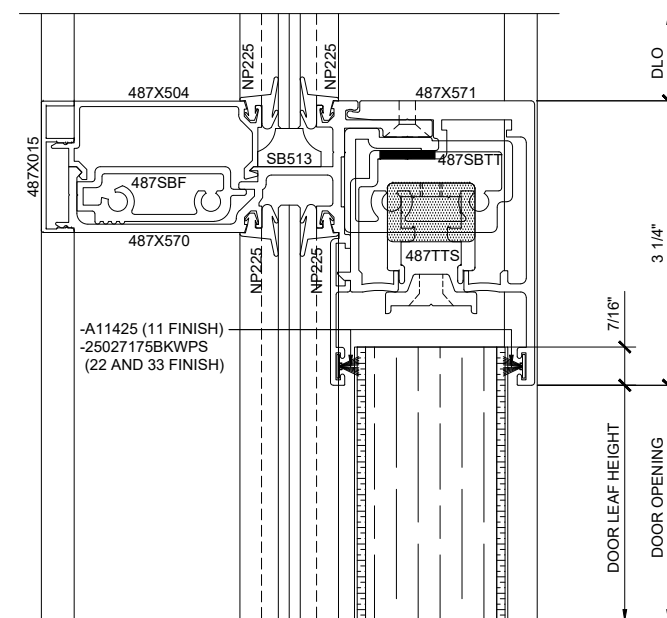
⑥ TRANSOM DETAIL AT SLIDER DOOR SIDELITE (DOOR OPEN)
