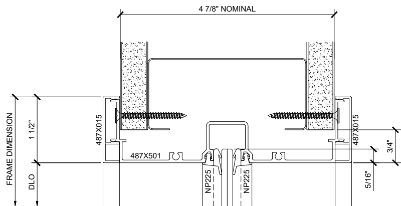
① SERIES 487 OPS TYP HEAD DETAIL AT INT. VERTICAL
