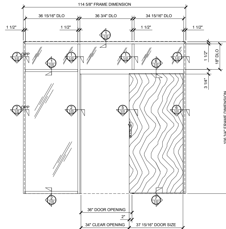
④ SINGLE SLIDER WITH TRANSOM AND SINGLE SIDELITE (OPEN)
