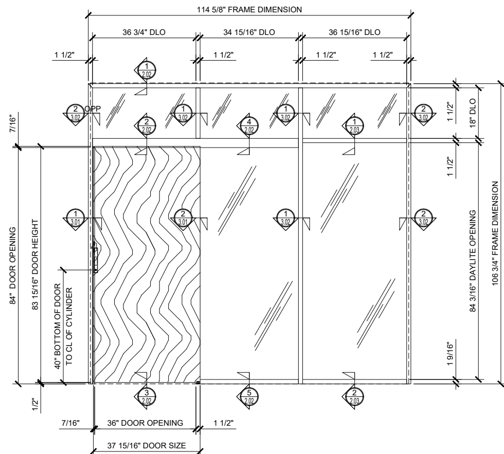
③ SINGLE SLIDER WITH TRANSOM AND DOUBLE SIDELITE (CLOSED)
