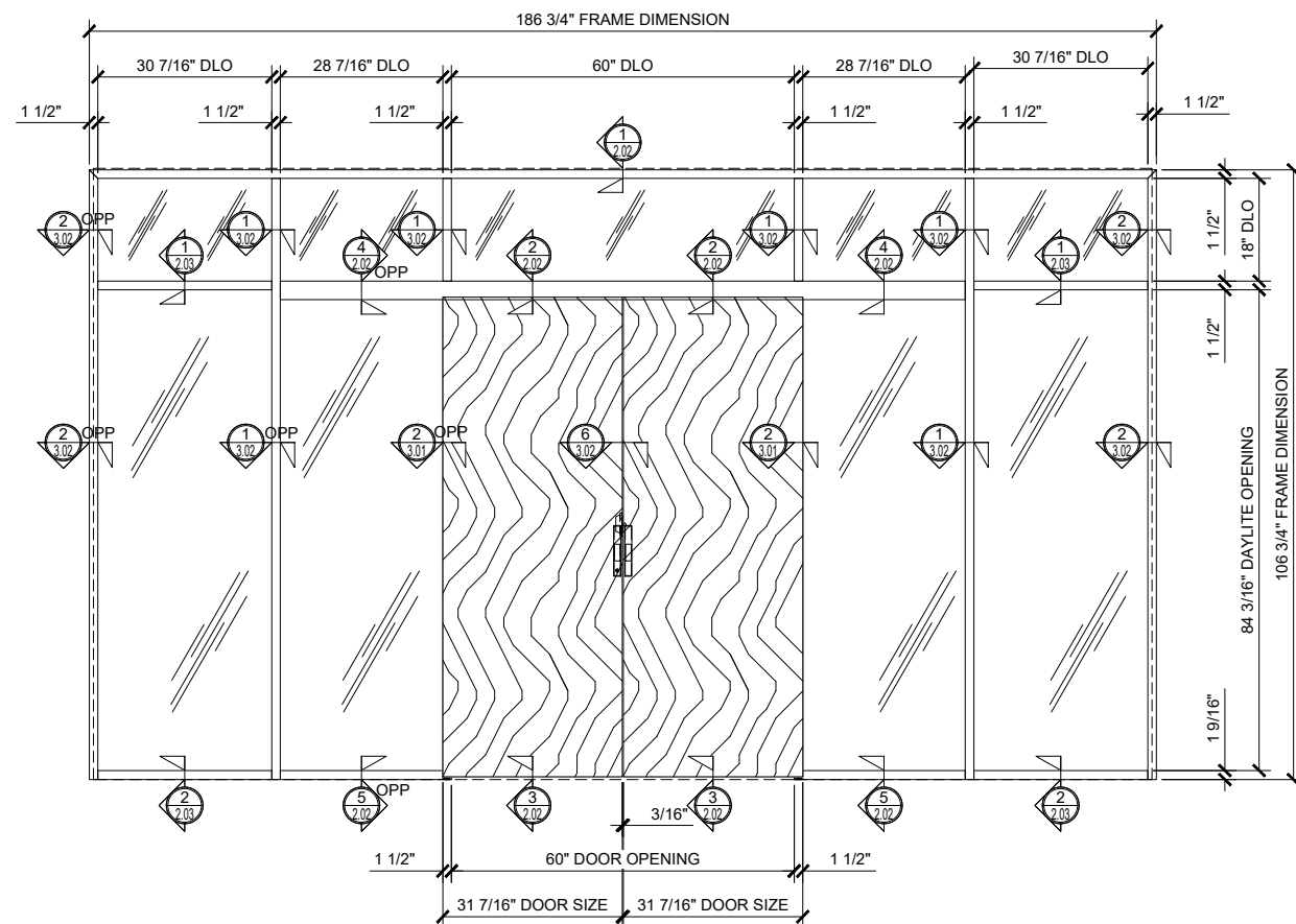
3 BI-PART SLIDER WITH TRANSOM AND SINGLE SIDELITES (CLOSED)
