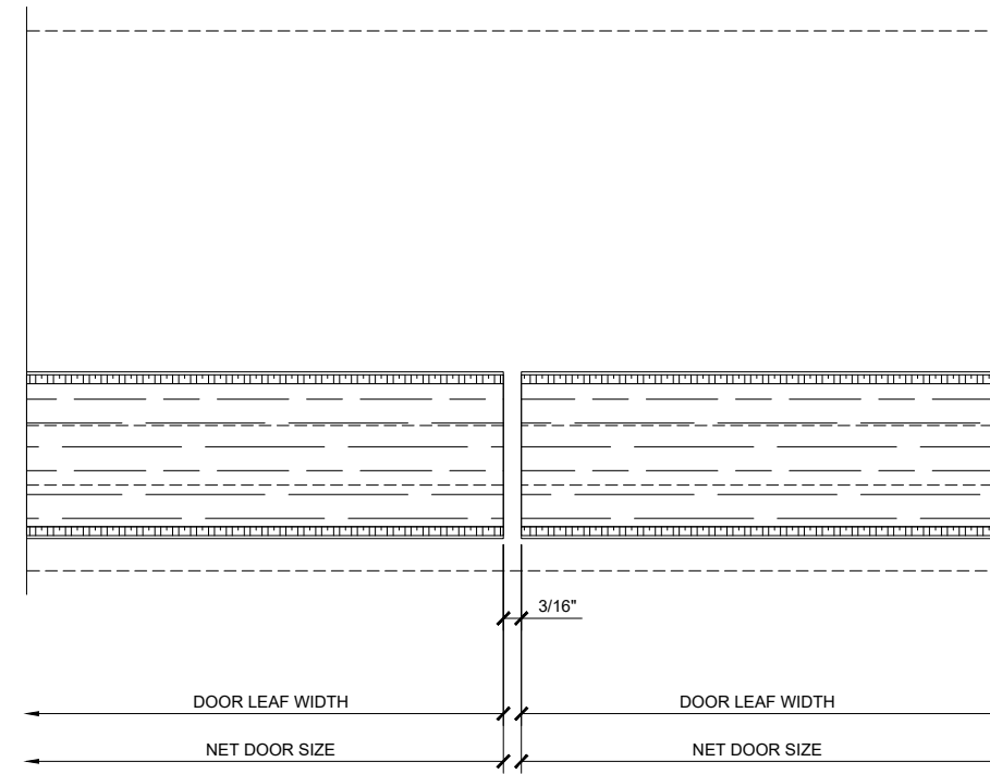
⑥ SERIES 487 OPS INTEGRATED SLIDER MEETING STILES AT DOOR PAIR DETAIL (CLOSED) ARCH REF: 1'-0"=1'-0"
