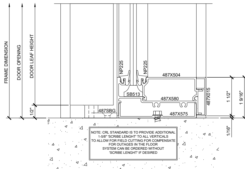
⑤ SILL AT SLIDER SIDELITE (DOOR CLOSED)
