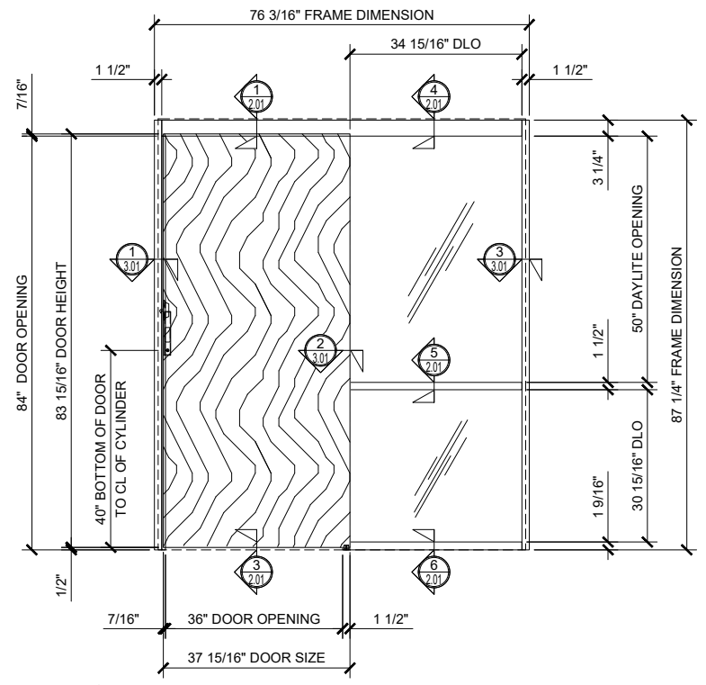
① SINGLE SLIDER WITH SINGLE SIDELITE (CLOSED) ARCH REF: NONE 3/4"=1'-0"
