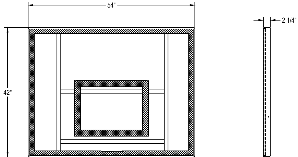
FRONT
