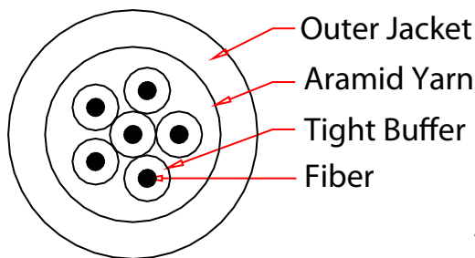
Cable Section
