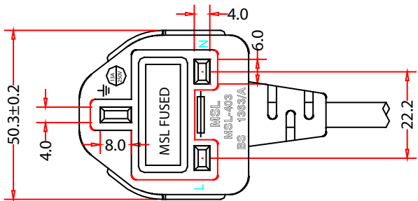
BS1363/A Male
