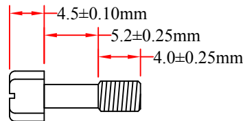
SCREW
