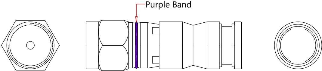
F-Pin Compression Connector Nickel Plated
