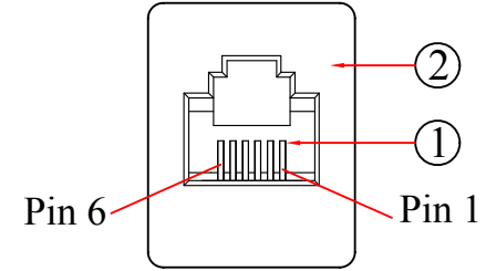
RJ12 Jack2
