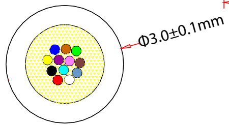
Cable Structure (Scale 10:1)
