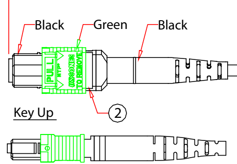
Cable Structure (Scale 10:1)
