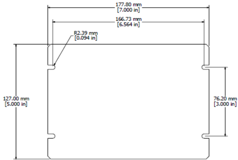
1431-12 OR 1431-12BK3 - VIEW FROM TOP (SOLD SEPERATELY)
