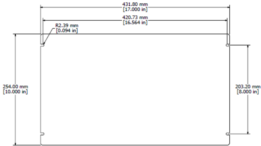
1431-30 OR 1431-30BK3 - VIEW FROM TOP (SOLD SEPERATELY)
