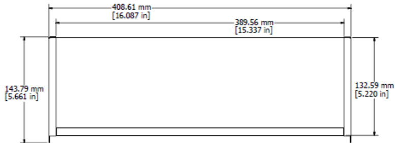
SIDE VIEW OF ASSEMBLY
