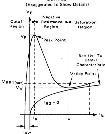
FIGURE 2 STATIC EMITTER CHARACTERISTIC CURVES
