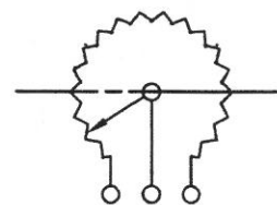
1 2 3 CIRCUIT
