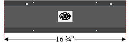
P-RMOD-9AB3C1B (1) spring reverb tank
