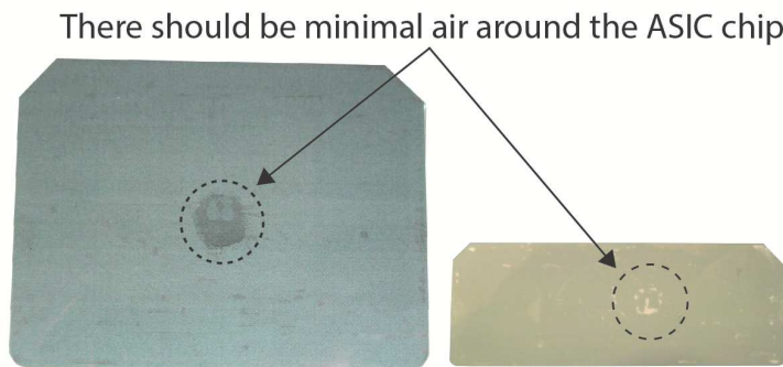
Figure 5 – Example of a properly installed mini tag
