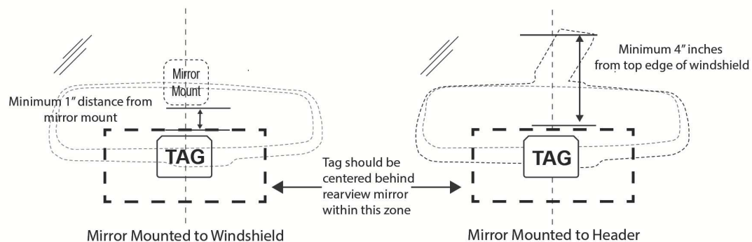
Figure 1 – Tag Location for Optimal Performance
