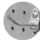
Hook #23 0502523 1-1/2" Right 22.5" Angle Hooks
