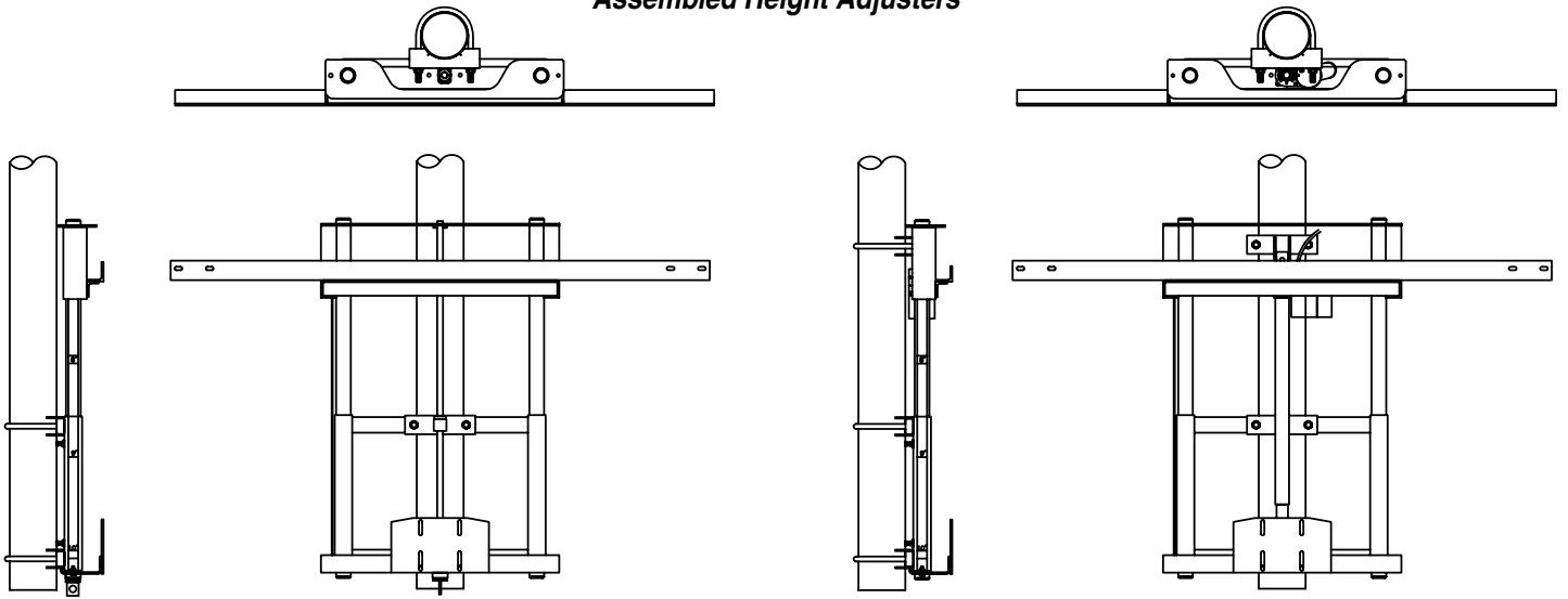
Rectangular Bank Motorized Height Adjuster
