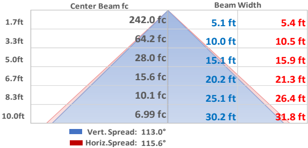
Illuminance at a Distance
