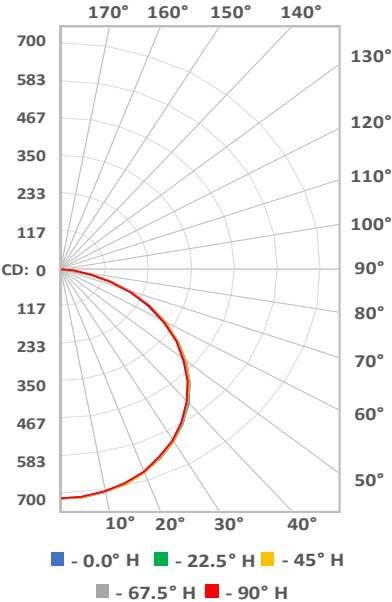
Polar Candela Distribution
