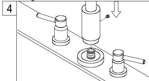
4. Insert spout escutcheon and insert spout onto spout shank. Secure the spout with the set screw and Allen wrench.
