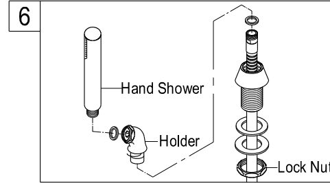
6. Slip hand shower holder assembly through the hole from top of the deck and secure by tightening from underneath with the locknut. Apply Teflon tape to threaded end of hose, attach hose to hand shower, and thread hose through hand shower holder.
