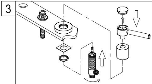
3. Hot and cold stem assemblies are easily identified by the red (hot) or blue (cold) bands, insert the stem assembly through the side holes from below making sure to have the bottom locknut and rubber washer threaded onto the stem assembly. When ready to install handle and handle flange, carefully remove the stem assembly locknuts while holding stem assembly from under the deck, slip on washer and thread escutcheon on to stem assembly, install the handle and adjust to a suitable height to allow sufficient space for handle to operate smoothly. Repeat for other handle and the diverter handle. Re-secure the bottom locknuts, make sure to align the direction of the handles before tightening stem. Hand tighten the valve body nut then gently tighten with a wrench.
