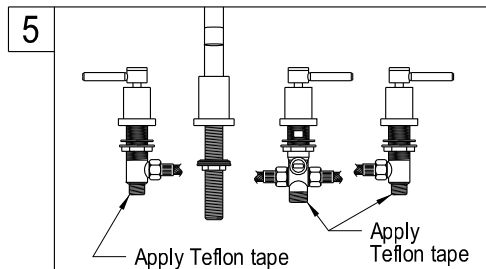
5. Apply Teflon tape to inlet shanks and connect supply lines.
