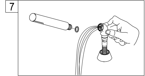
7. Remove hand shower by unscrewing the sprayer in a counter clockwise direction, turn on both hot and cold valves and let water run for at least one minute, this will clear any debris left in the line.
