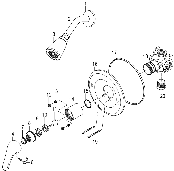
Cartridge: KBRP521C
