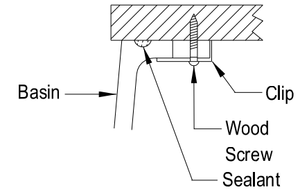
Detail for Wood Countertop
