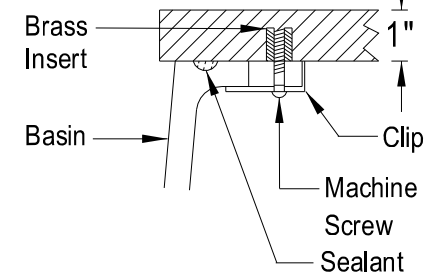
Detail for Solid Countertop
