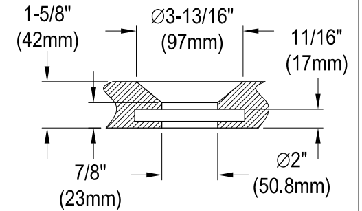
Drain Hole Size Scale (3:1)
