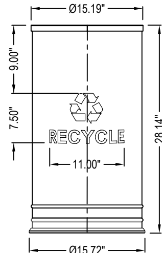
BOTTOM VIEW
