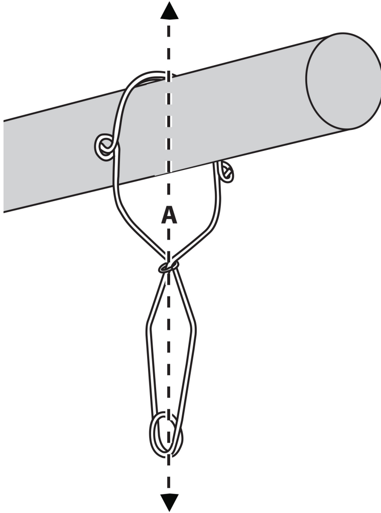
Figure 3: Load Direction of Wire Form Anchor A Permissable Load Direction Only on Major Axis of Anchor
