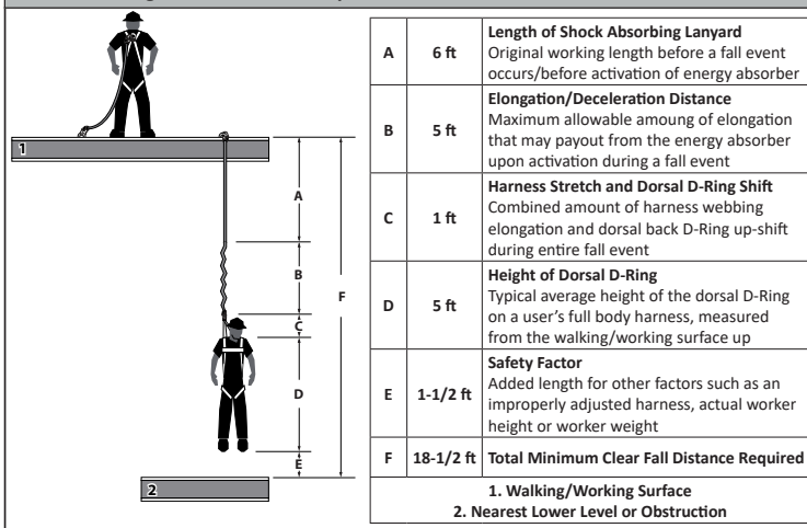
Figure 1- Minimum Required Fall Clearance - Foot Level Tie Off
