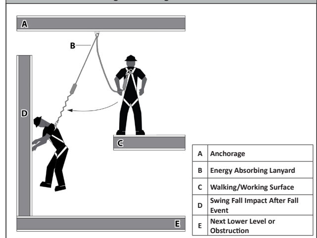
Figure 2- Swing Fall Hazard
