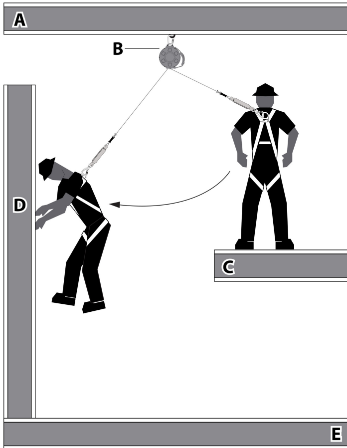
Figure 9B: Swing Fall Hazards Non-Leading Edge
