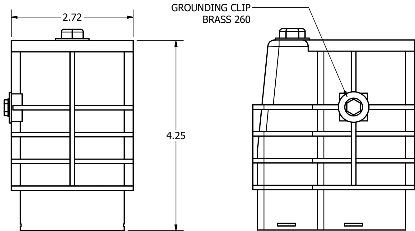
ANCH-1 SAFTRON ANCHOR SOCKET
