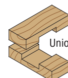
Tongue and groove joint
