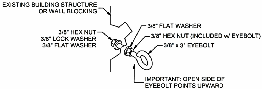
Figure 1: Standard Building Attachment - For Metal Structure and Wood Blocking
