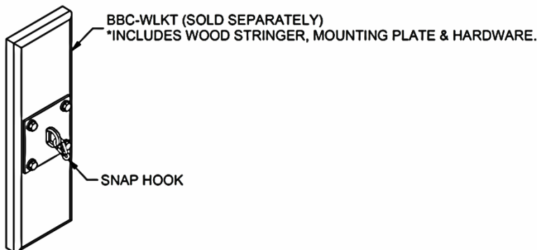
Figure 3: Optional Wall Mounting Kit – For CMU and Studded Walls (Alternate Wall Anchors Required)
