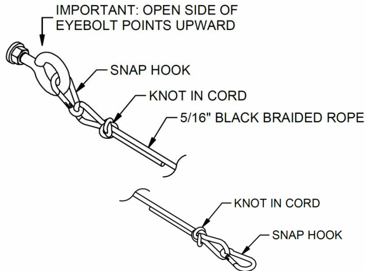
Figure 4: Fixed End Support Lines (Line Length Base on Desired Distance off the Wall)
