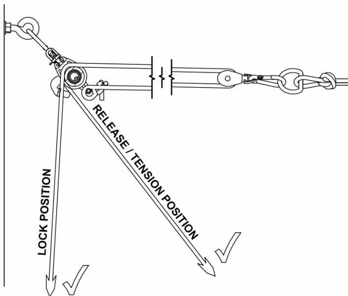
Figure 7: Assemble Suspended Net Leads
