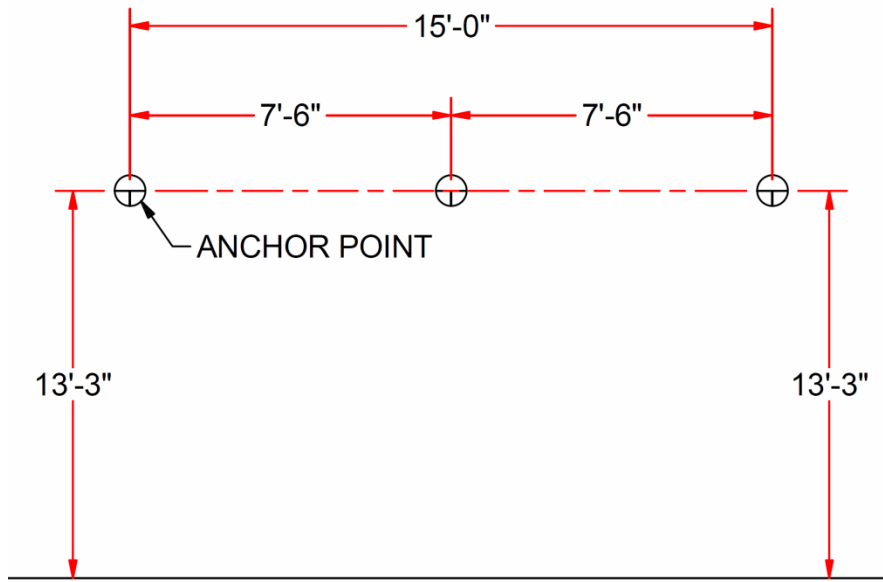
Anchor Point Locations on Building Wall (Both Ends)
