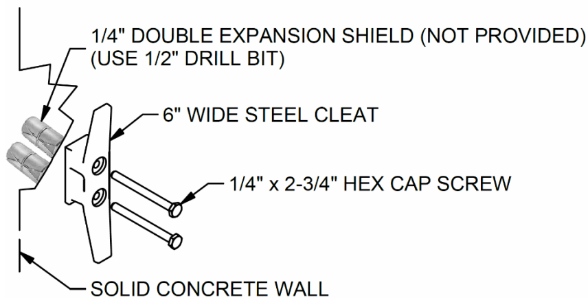
Figure 9: Standard Building Attachment on Fixed End - For Solid Concrete Walls (Double Expansion Shield Not Provided)
