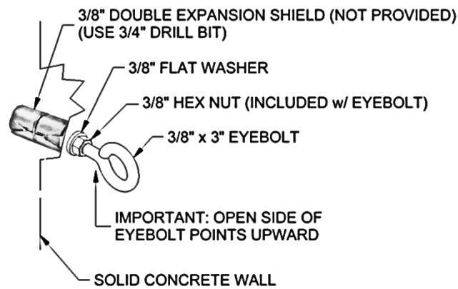
Figure 2: Standard Building Attachment - For Solid Concrete Walls (Double Expansion Shield Anchors Not Provided)
