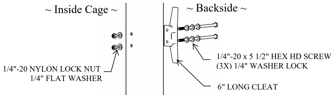
FIGURE: 4 – TYP POLE HARDWARE
