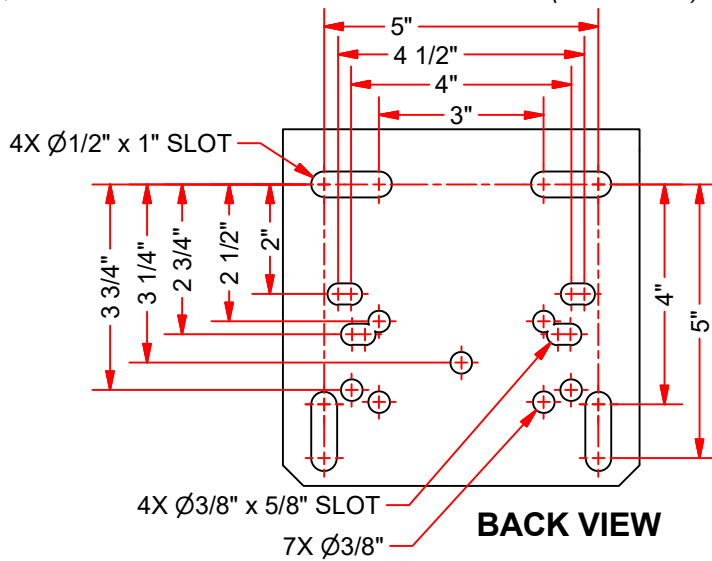
PIG TAIL NET ATTACHMENT SYSTEM (12 PLACES)
