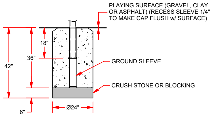
NON-SAND FOOTING (SHOWN ABOVE)
