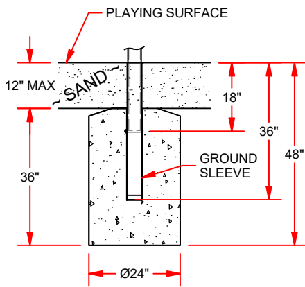
SAND-FILLED FOOTING * DEPENDING ON SAND DEPTH (SHOWN ABOVE)
