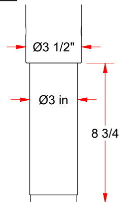
FOOTING DETAIL
