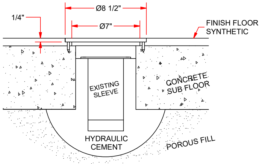
TYPICAL INSTALLATION IN A SYNTHETIC FLOOR
