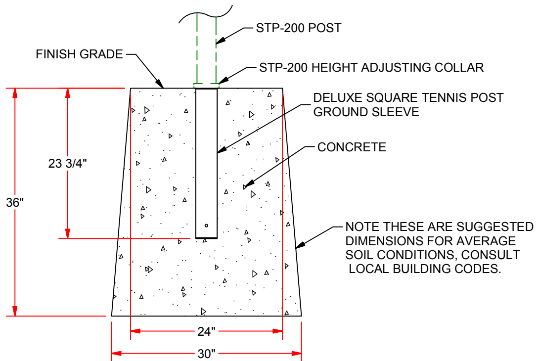
TYPICAL FOOTING DETIAL
