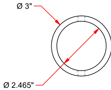
TOP VIEW (HIDDEN SHOWN)
