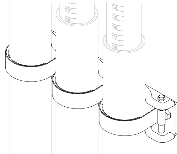
WALL RACK INSTALLED WITH UPRIGHTS
