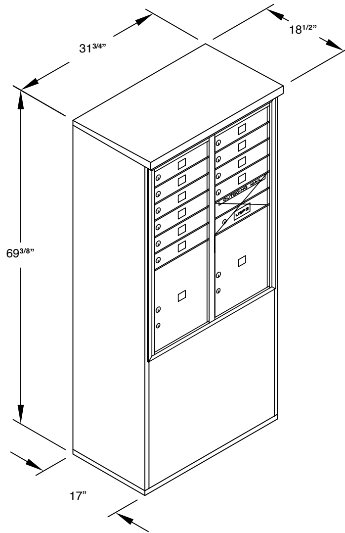
MODEL #3911D-10 - FRONT LOADING
